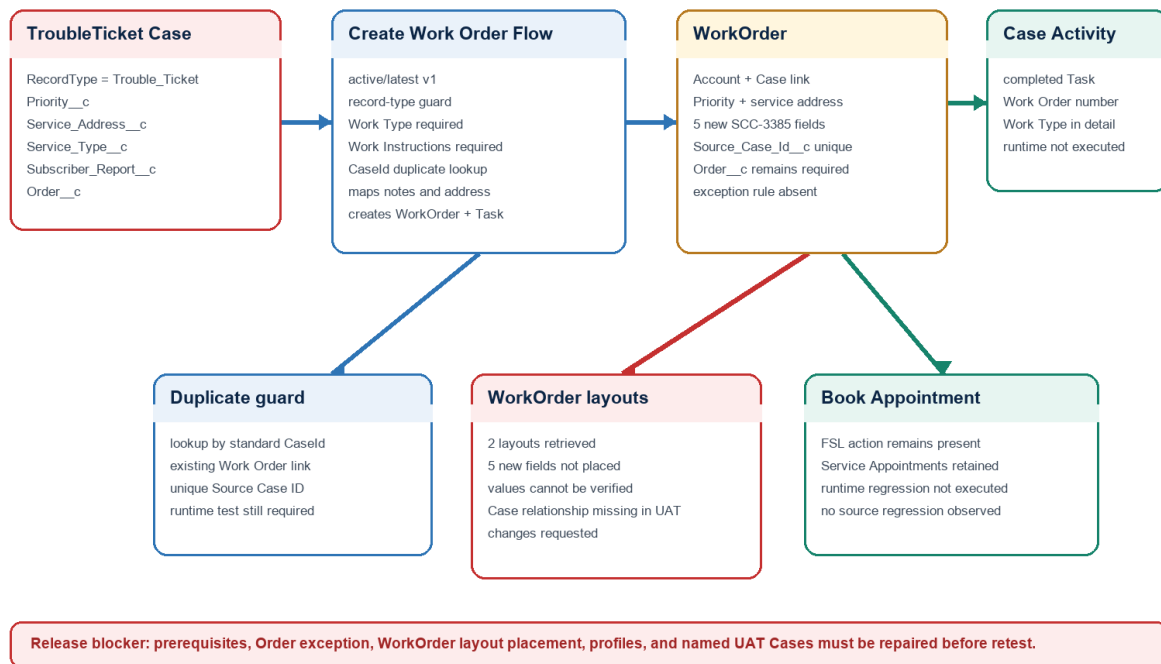
Figure 2. SCC-3385 Work Order creation and dependency model
