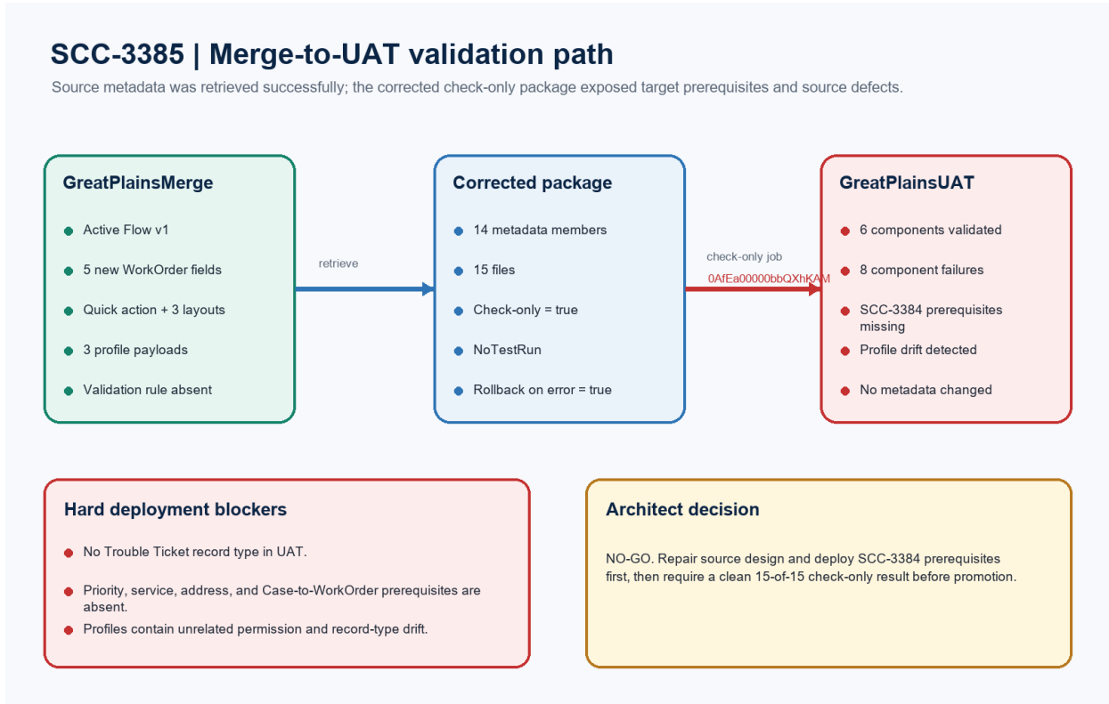
Figure 1. SCC-3385 Merge-to-UAT validation path
